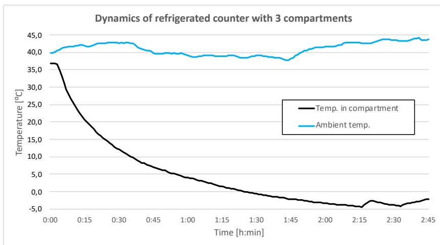
Dynamics of refrigerated counter with 3 compartments
