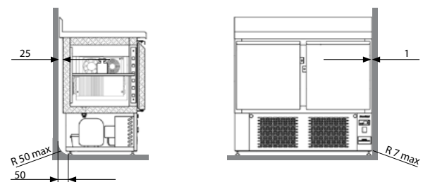
Counters with bottom engine compartment
