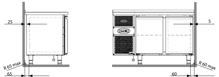
Counters with side engine compartment
