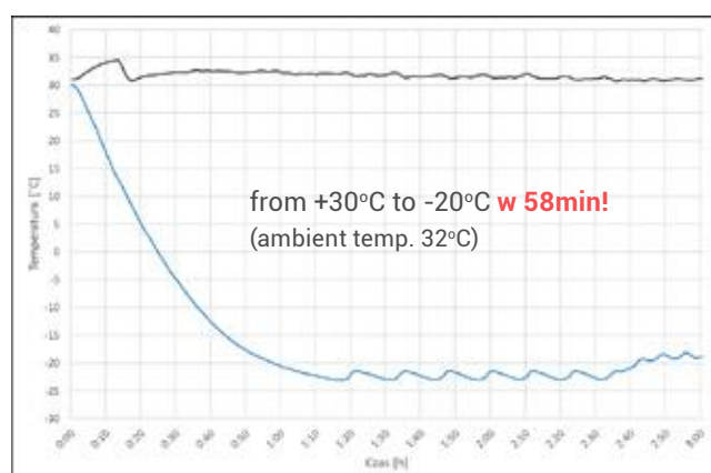
Dynamics of freezer in STANDARD line
